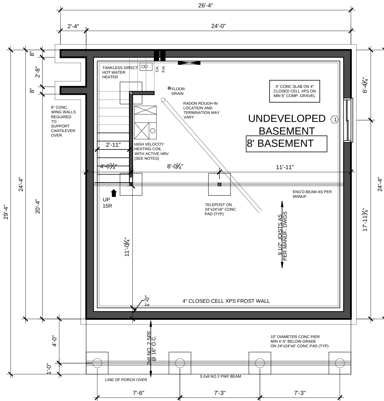
FOUNDATION PLAN SCALE: 3/16"=1'-0"
