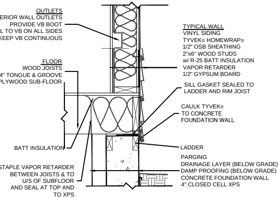
BASE OF WALL AT STAIR DETAIL
