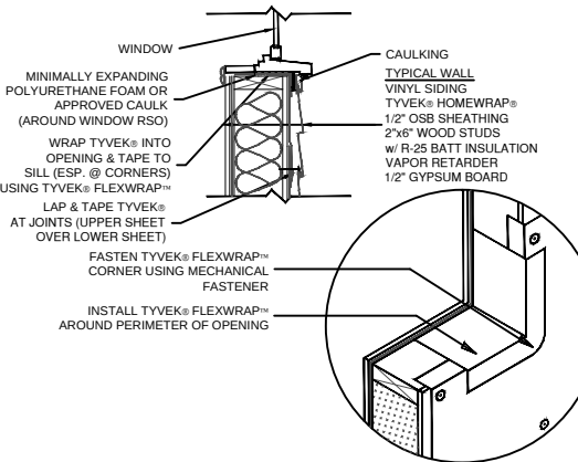
WINDOW SILL DETAIL
